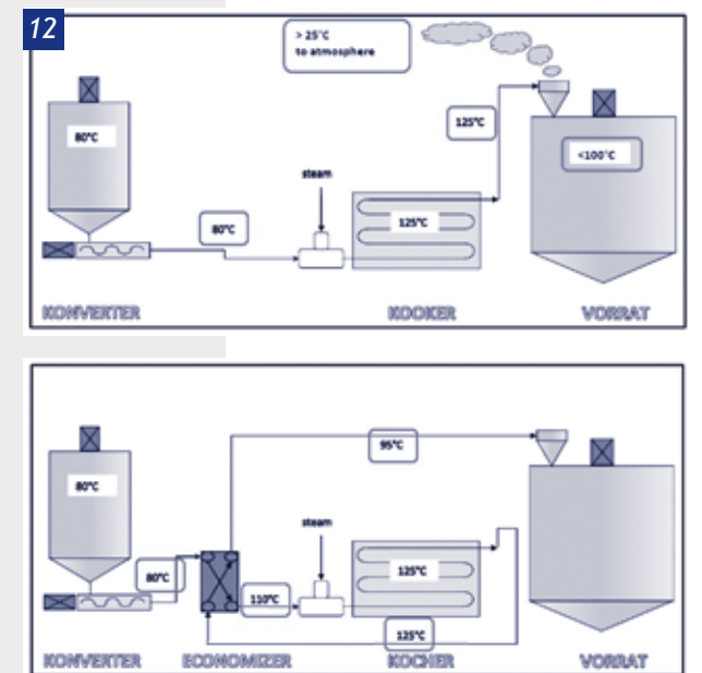
12 Schematic representation of the new GAW starch preparation process in the form of the Starch Economizer
